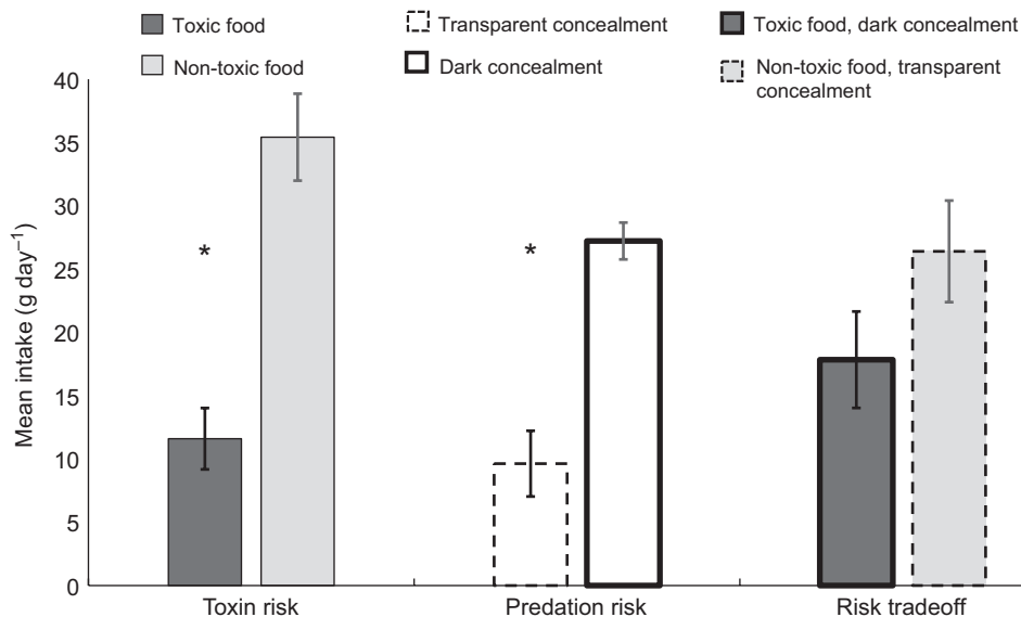
Figure 1. Daily intake (mean \pm SEM, grams dry weight day -1 ) of food by pygmy rabbits during three choice treatment trials. Dark gray bars represent foods with high food risk (high PSM), dashed borders represent concealment with high predation risk (low concealment), and asterisks denote significance between the two treatments within a trial. The food risk trial provided rabbits the choice of PSM-containing food (5% cineole by dry weight) or PSM-free food (no cineole added) under constant concealment. The predation risk trial provided rabbits with the choice of PSM-free food under high predation risk (transparent concealment) or under low predation risk (dark concealment). The risk tradeoff trial provided rabbits with a choice of PSM-containing food under low predation risk or PSM-free food under high predation risk.
