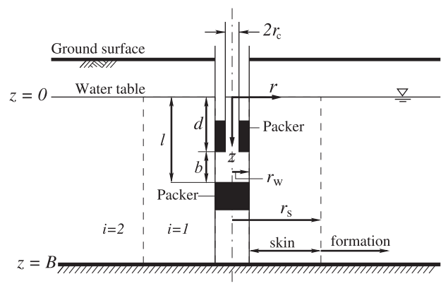
Fig. 1. Schematic of the slug-test problem flow domain.
