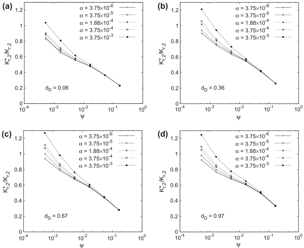
Fig. 7. Semi-log plot of K_{r,2}^*/K_{r,2} , against the dimensionless parameter \psi = (r_w/b) \sqrt{K_{z,2}/K_{r,2}} , for different values of the dimensionless parameter \alpha = 2bS_{s,2}(r_w/r_c)^2 , at depths of (a) d_D = 0.06 , (b) d_D = 0.36 , (c) d_D = 0.67 and (d) d_D = 0.97 , to the top of the test interval.
